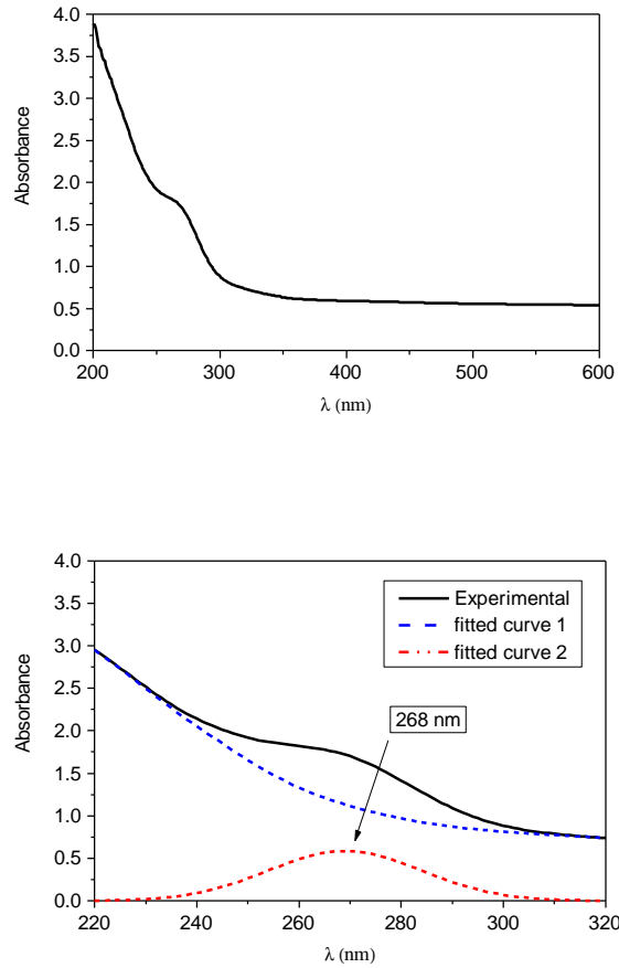
Figure 3. UV absorption spectrum of nanometer-sized bismuth aqueous solution. ((a)—top fig: the real experimental spectrum; (b)—bottom fig: resolved curves).
