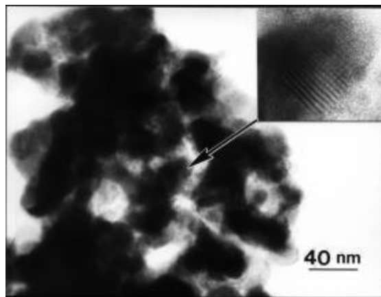
Figure 2. Transmission electron micrograph of bismuth nanoparticles prepared via the reverse microemulsion method. The top-right micrograph is an enlarged lattice image.
