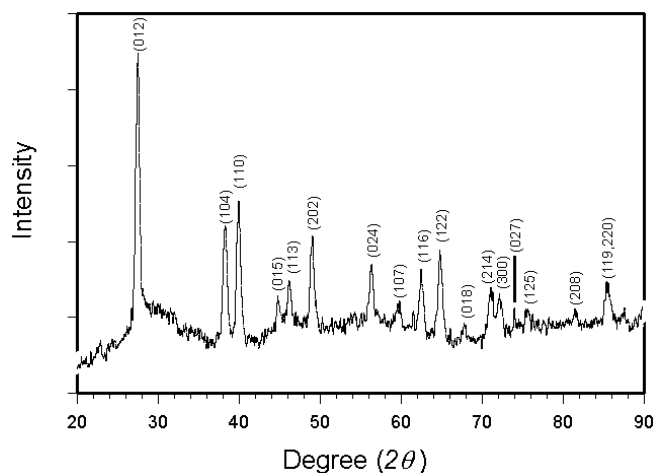
Figure 1. XRD traces of the bismuth nanoparticles prepared via the reverse microemulsion method.
