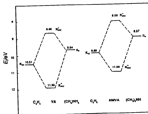
Fig. 2 Correlation diagram for the experimental vertical ionization potentials of vinylamine, N -methylvinylamine, ethene, propene, methylamine and dimethylamine. The value for propene was taken from ref. 20 and those for ethene and the alkyl amines were taken from ref. 21.
