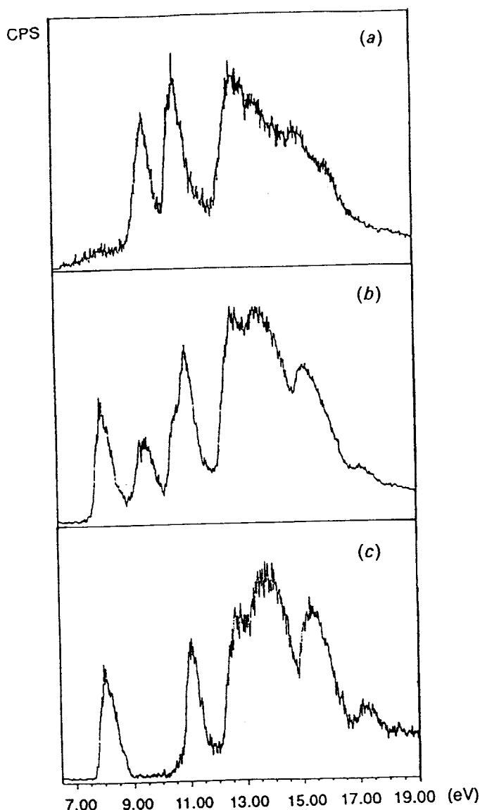
Fig. 1 He(I) photoelectron spectra. (a) Spectrum of MEIM; (b) spectrum of mixture (NMVA + MEIM) released from the cold-trap at -36\text{ }^{\circ}\text{C} ; (c) spectrum of NMVA.
